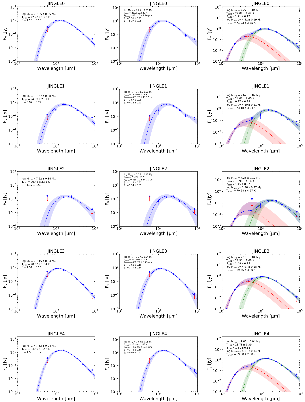
Figure 1. FIR SED of the galaxies of the JINGLE sample, fitted with the hierarchical approach using the three models: SMBB (left panel), BMBB (middle panel) and TMBB(right panel). The shaded regions show the lower and upper 1-sigma uncertainties on the SED models, defined by taking the maximum and minimum flux values of the models with likelihood values in the highest 68th percentile.
